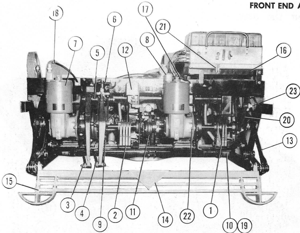
82-70-1500 FRONT END ASSY.
